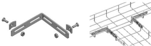
Connector Kit (44994)
