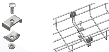
Wall Mount Support Kit (449D5-0100)
