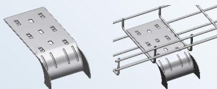
Drop Out (44995-0400)
